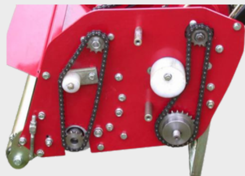
Chain driven cutting cylinder and rear roller, with nylon chain adjusters
