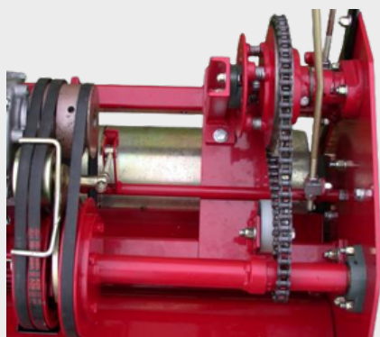
Heavy duty chain and belt driven clutch
