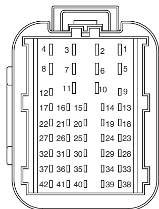
J6 Connects to Mower Harness
