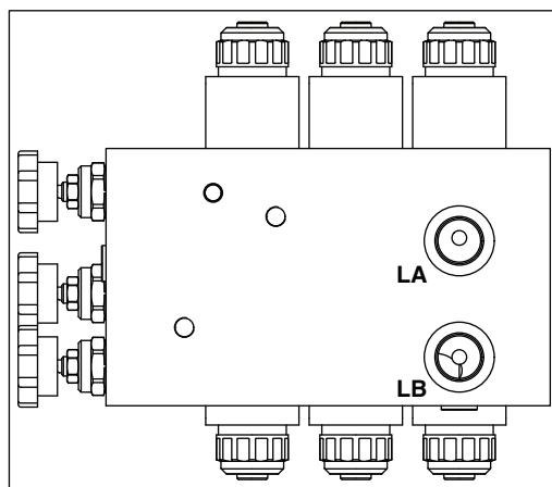
Rear Reel Valve Viewed from Bottom
