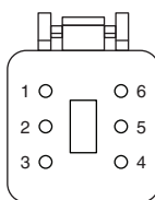
Traction Pedal ( U5 ) To 7 Gang Harness ( J16 )
