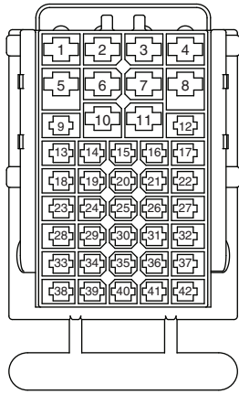
J6 Connects to Engine Harness
