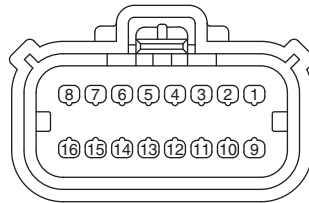
J8 Connects to DPF Harness
