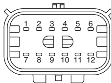
J10 Connects to Mower Harness
