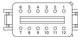
MCU J1 (U18) (Black)
