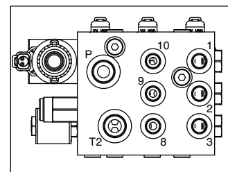
Lift Valve Viewed From Front
