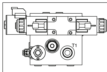
Lift Valve Viewed From Right
