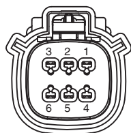
To Armrest Harness ( J15 )
