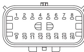
J8 Connects to Mower Harness
