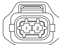
Fuel Injector #3 (U15)
