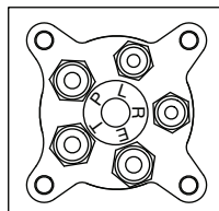
Steering Valve Viewed From End Of Valve
