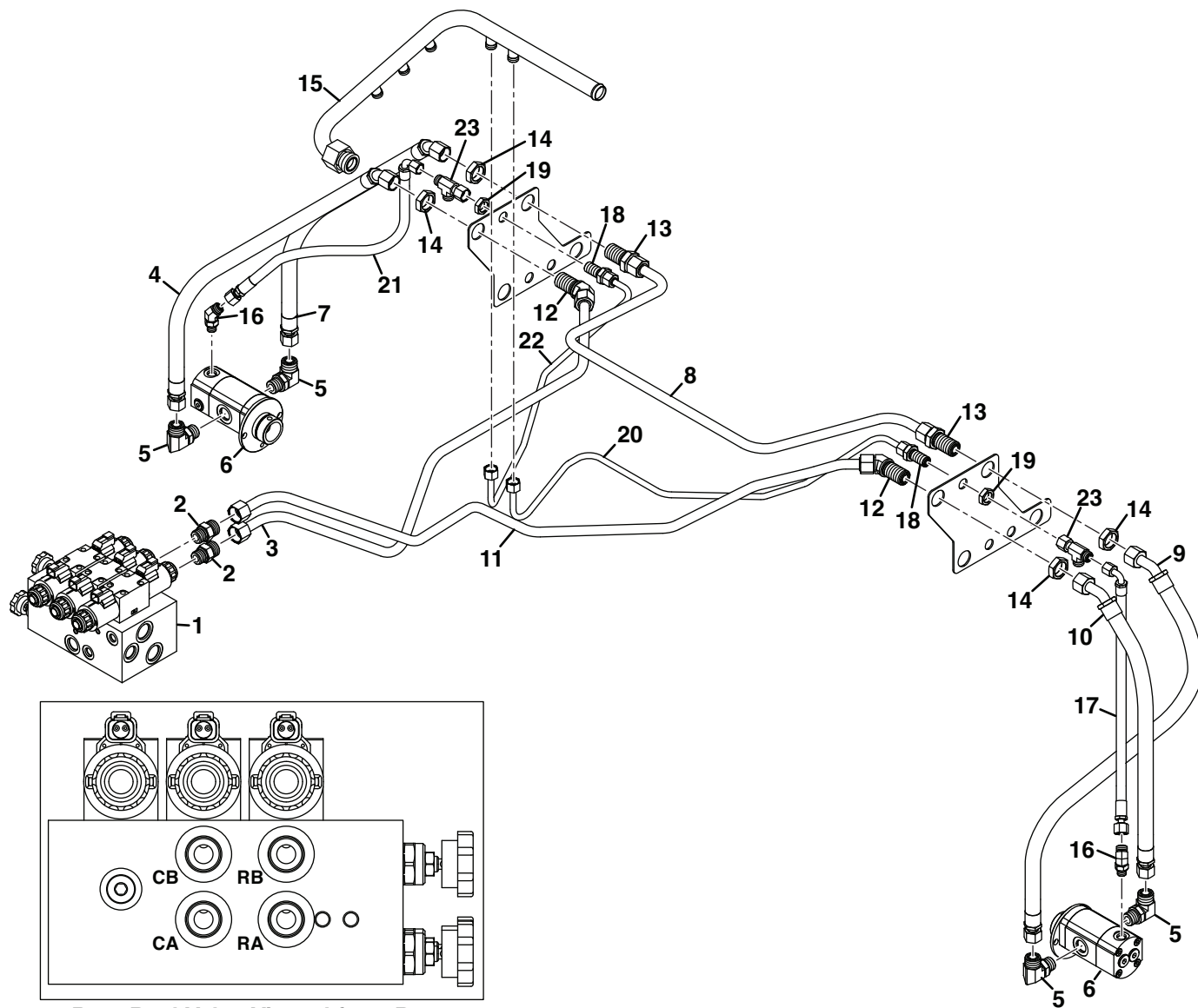
Rear Reel Valve Viewed from Rear
