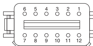
MCU J3 (U18) (Grey)
