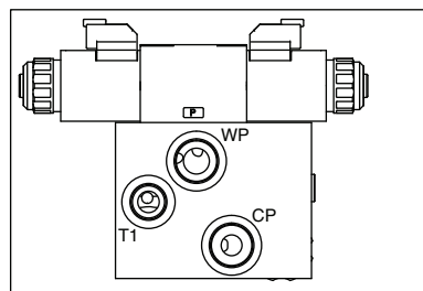
Rear Reel Valve Viewed From Left
