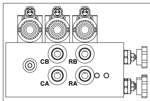
Rear Reel Valve Viewed from Rear
